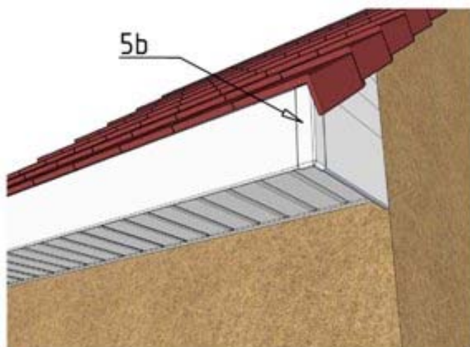
Figure 9a – Pose horizontale
